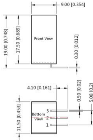
K78XX-L
