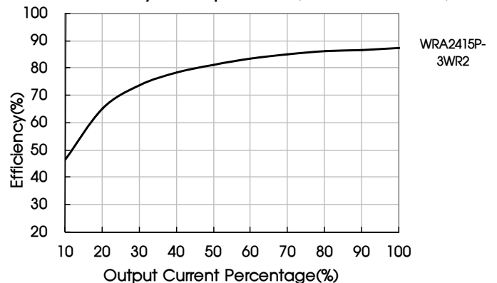
Efficiency Vs Output Load( V_{in}=V_{in-nominal} )
