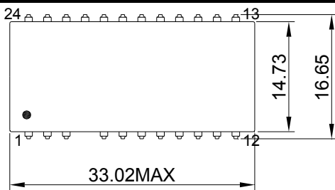
Markings and dimensions
