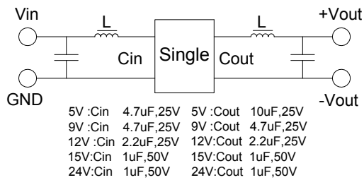
Recommended Test Circuit
